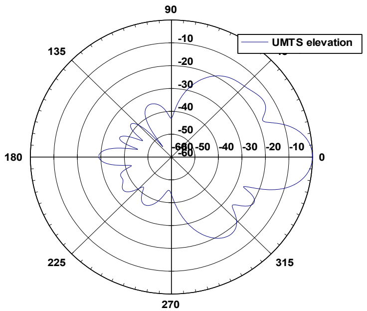
Elevation Pattern
