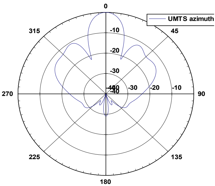
Azimuth Pattern
