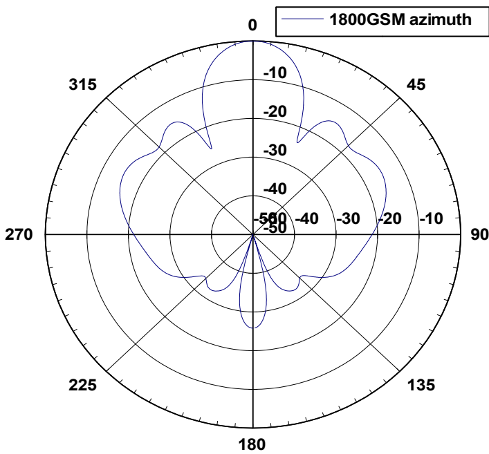
Azimuth Pattern
