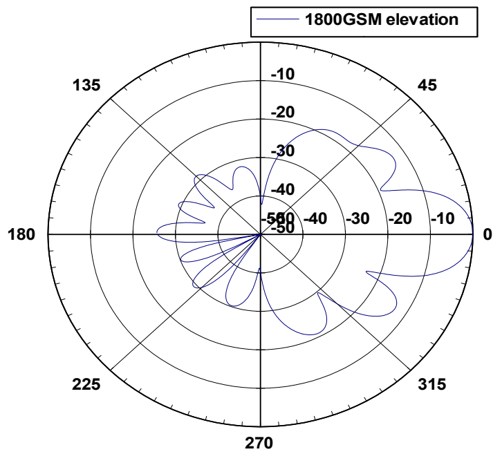
Elevation Pattern
